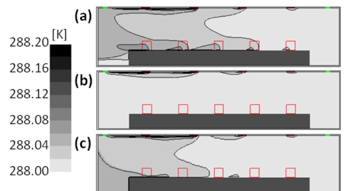
Fig.4 Temperature fields, (a)True value, (b)the value calculated without VCA, (c)Estimated value
