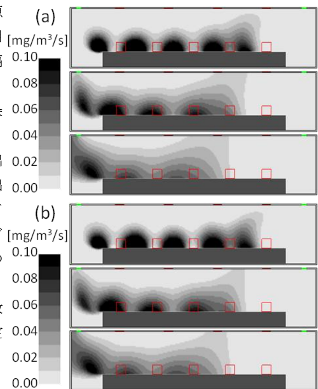
Fig.2 Contamination field, (a)True value, (b)Estimated value
